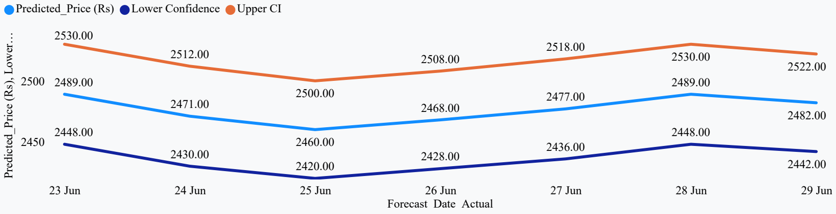
Prediction with Confidence Interval
